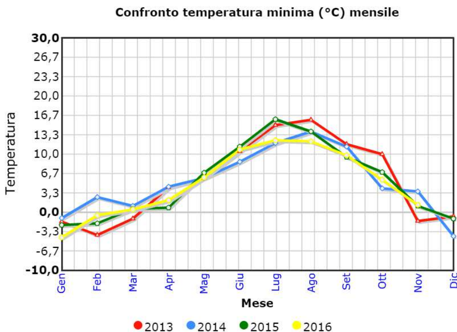
Figura 14 – Temperature minime mensili (2013-2016)
